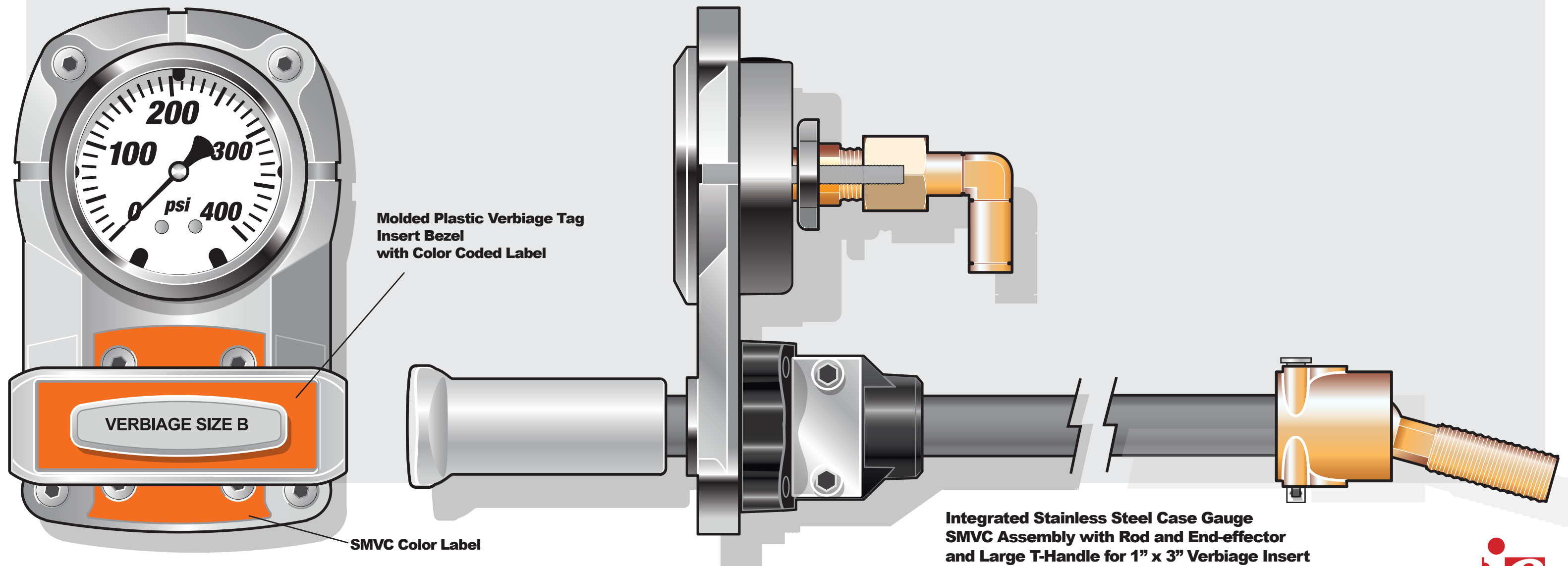
Swoop Series Side Mount Valve Control with Large T-Handle for 1" x 3" Verbiage Insert
