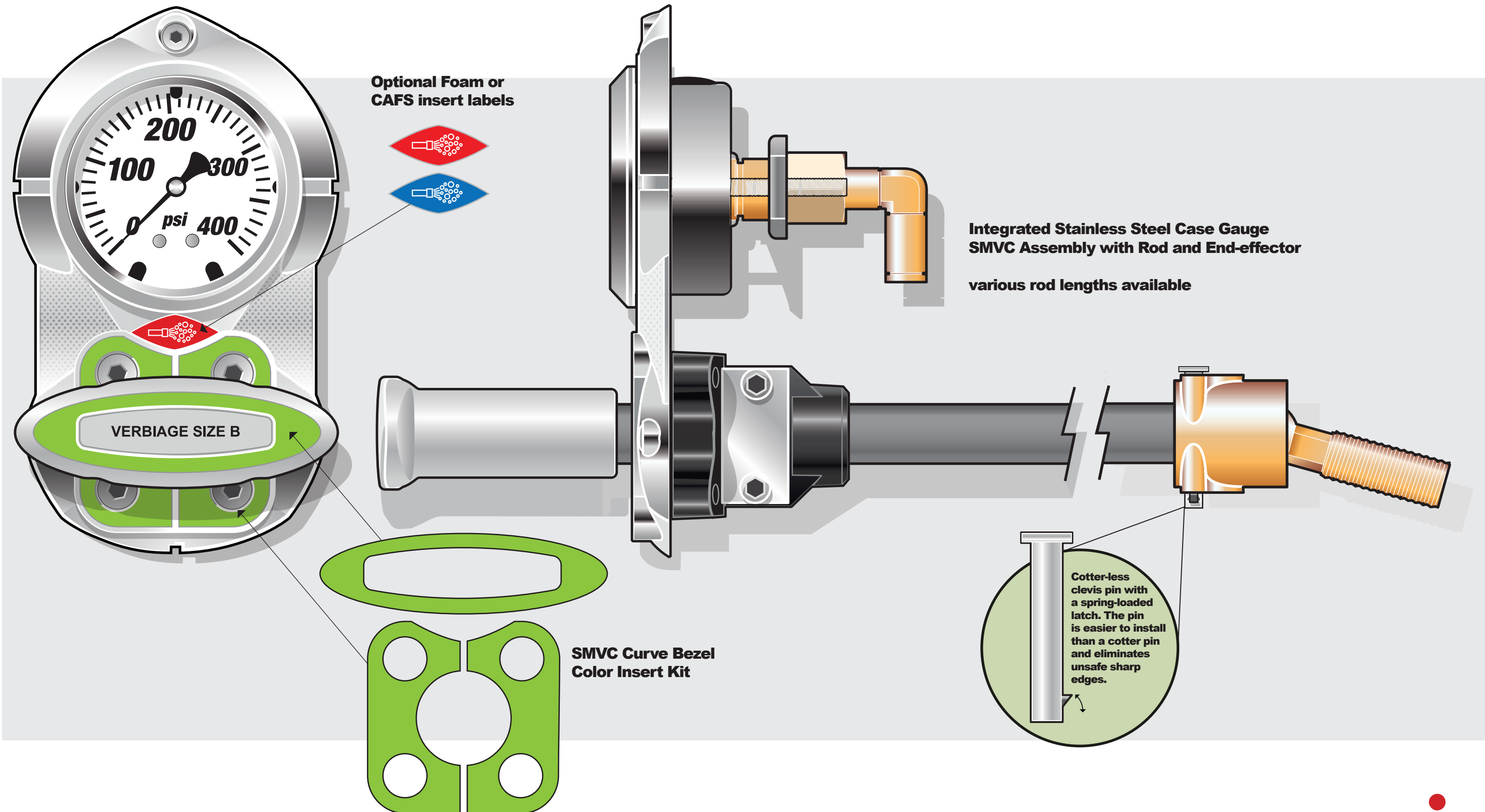
Curve Series Integrated Side Mount Valve Control
